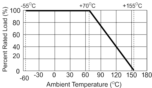
Derating Curve
