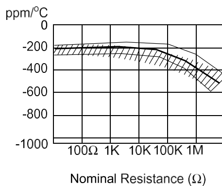
Temp. Coefficient
